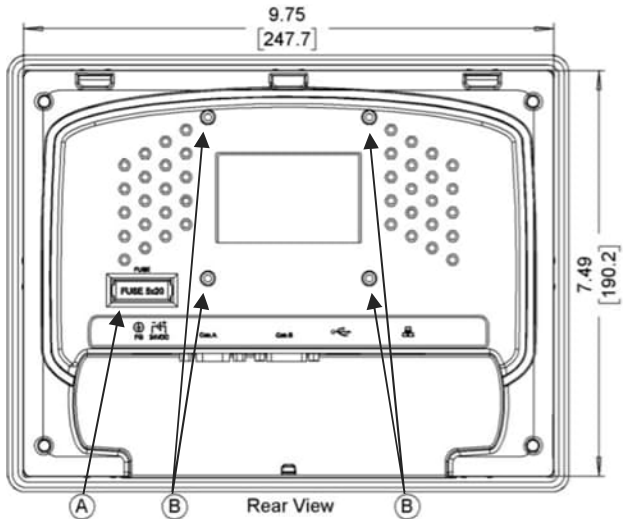
Rear View
